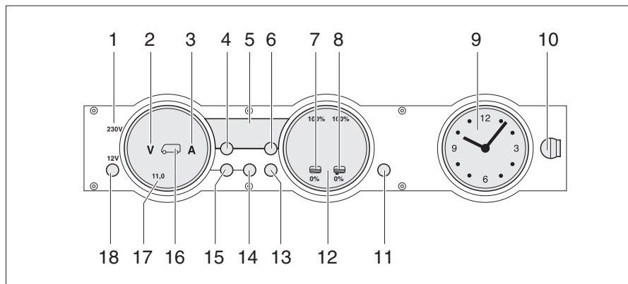
Rys. 245 Panel MP 20-T
