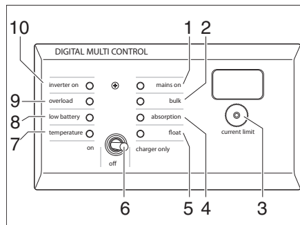
Rys. 239 Panel IT 992
